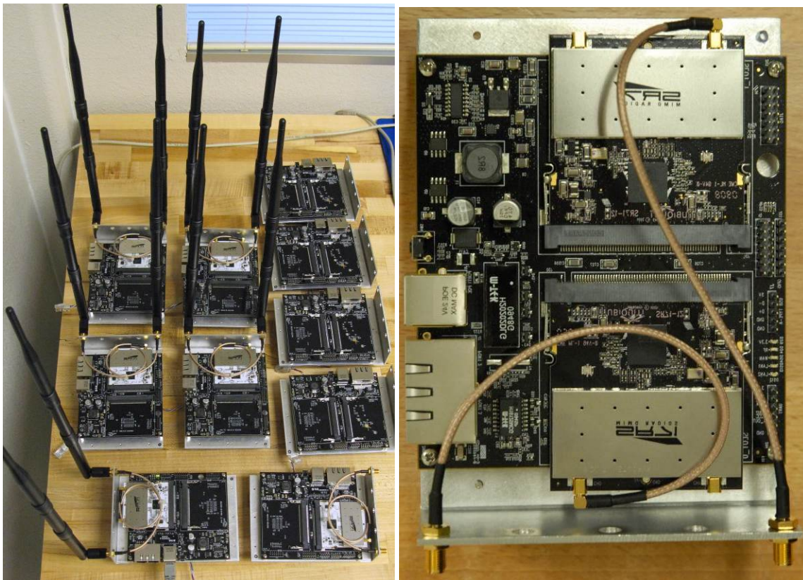
Figure 4.6 AHMCT 5.8 GHz mesh network experiment setup
