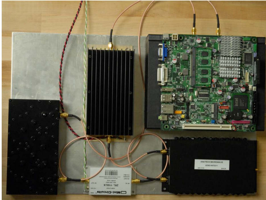
Figure 4.1 OpenBTS base station hardware implementation at AHMCT
